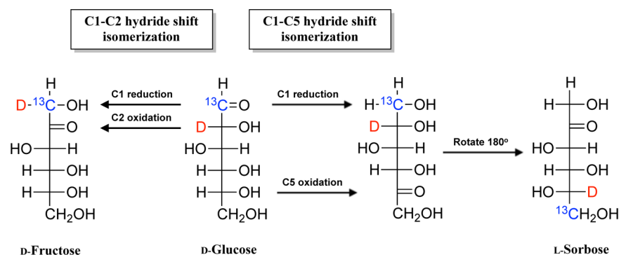
Scheme 1. Parallel Reaction Scheme for Glucose–Fructose and Glucose–Sorbitose Isomerization Mediated by Lewis Acidic Ti 4+ Centers in Ti-Beta a
